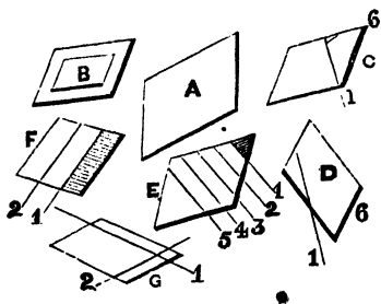
Fig. 192. Iodide of Mercury in Rhombic Prisms.
